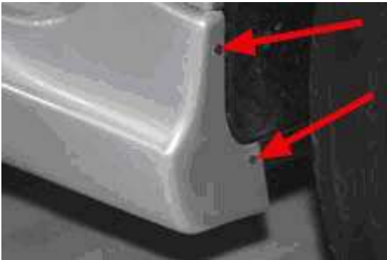
Photo 3: Positions of two mounting screws at the front of each Side Skirt
